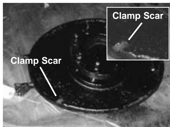
Figure 11: Recovered Inspection Manway Cover
